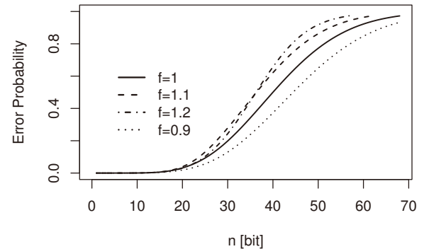
Fig. 1. Lower bounds for Eve's decoding error probability in the case where she gets the secret key K_s after her measurement for CPPM quantum signals
